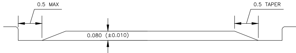
SECTION B-B
